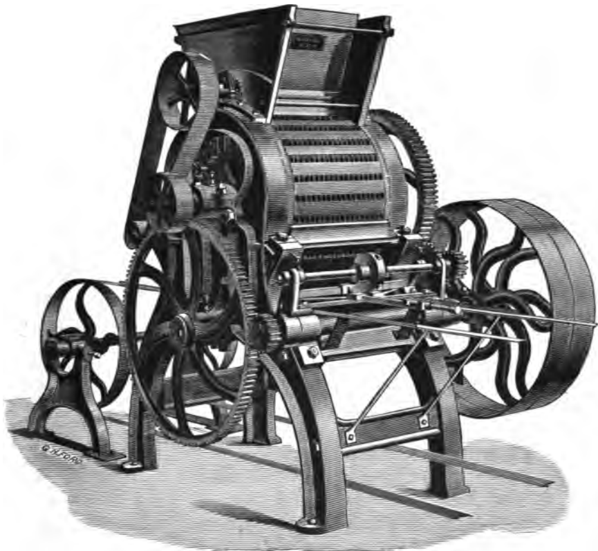
FIG. 39.—HERSEY CUBE-SUGAR MACHINE
